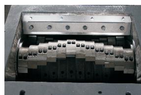
RG-26EA/36EA 爪刀型 Staggered blades type
