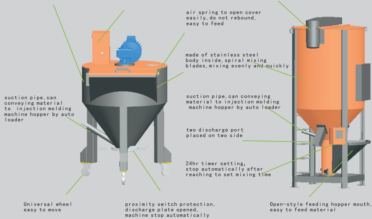
RSM80~RSM260 smaller spiral mixers
