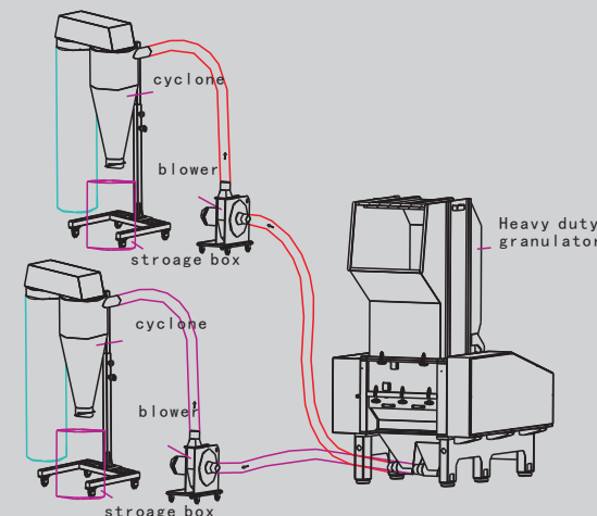
Heavy duty granulator Installation diagram ----blower system
