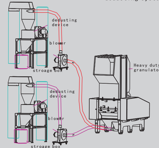
Heavy duty granulator Installation diagram ----blower system +dedusting system
